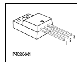
PG-TO220FP
